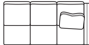
560-080 RSF Sofa 78 W 38 D 35 H 29 AH 21 SH
